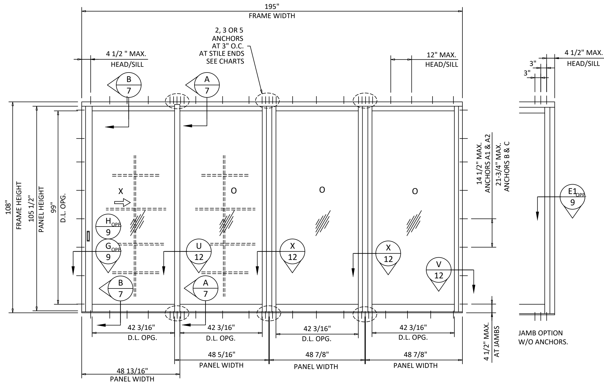
ELEVATION X000 OOOX/XOO/OOX CONFIGURATIONS ARE SIMILAR
