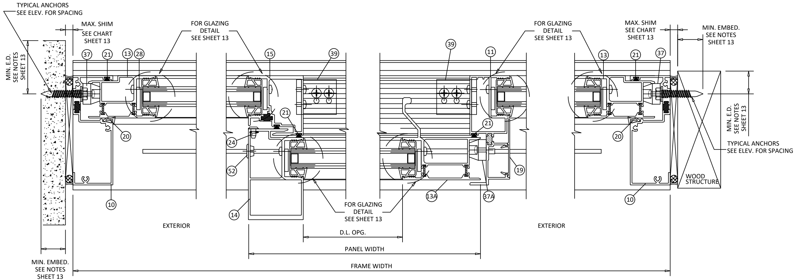
M HORIZONTAL SECTION JAMB - THROUGH FRAME FIXED PANEL - STANDARD SILL
