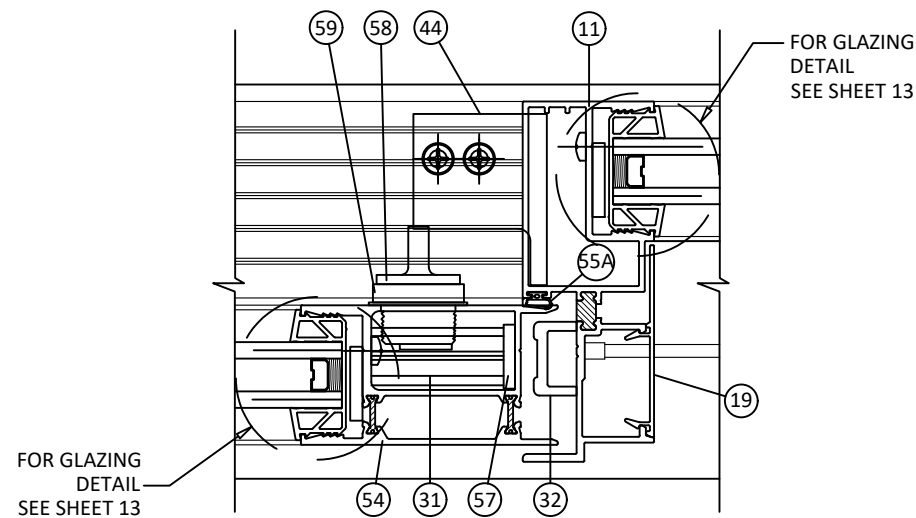
Q1 11A HORIZONTAL SECTION INTERLOCK OPERABLE TO FIXED WITH LOCKING HARDWARE LOW SILL
