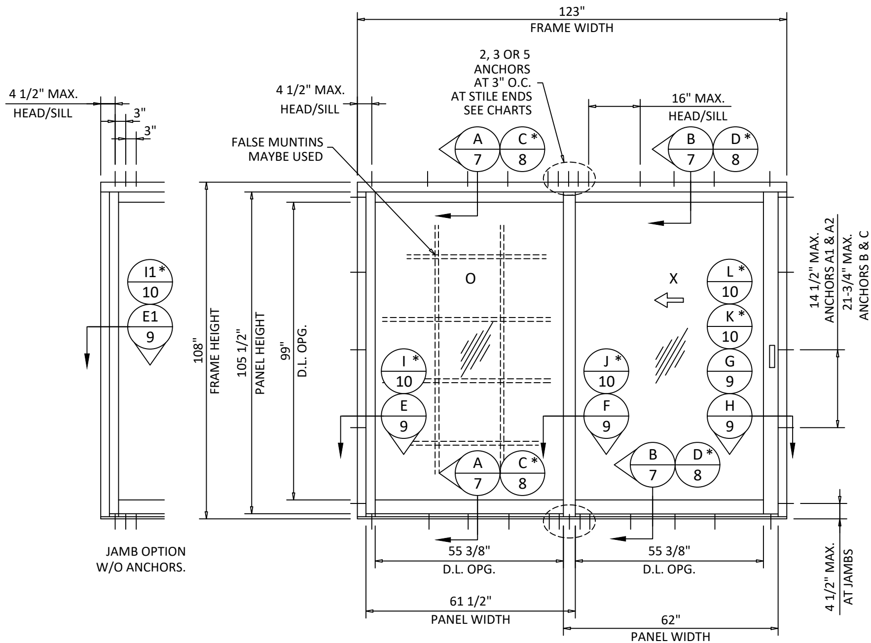
ELEVATION OX/XO *OPTIONAL FOR LOW SILL
