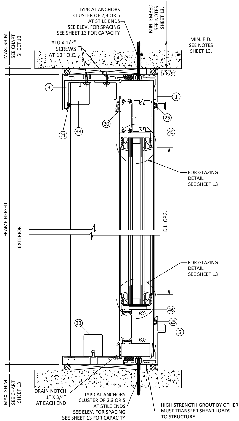
A 7 VERTICAL SECTION FIXED PANEL - STANDARD SILL
