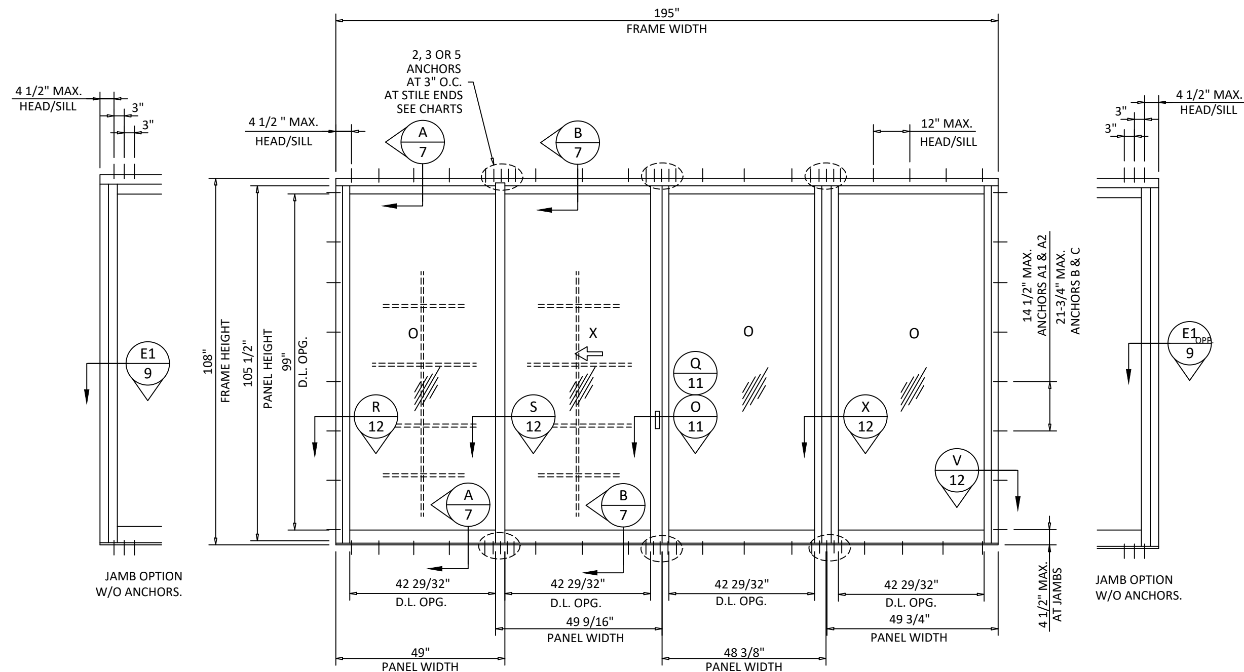
ELEVATION OXOO OOXO CONFIGURATION IS SIMILAR
