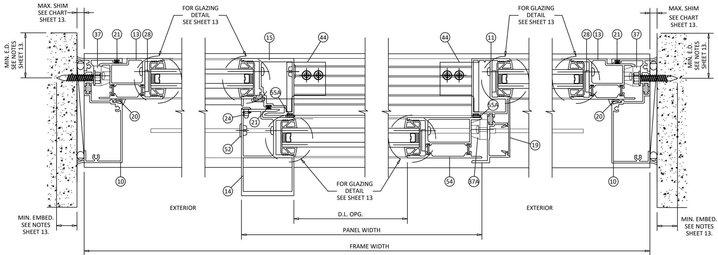
M1 11A HORIZONTAL SECTION JAMB - THROUGH FRAME FIXED PANEL - LOW SILL
