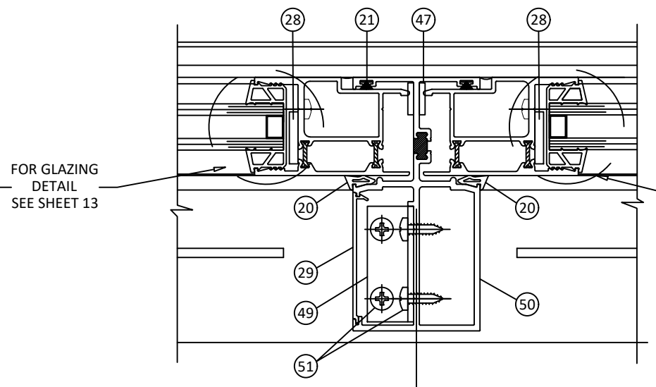
X HORIZONTAL SECTION 12 MULLION - FIXED TO FIXED STANDARD SILL
