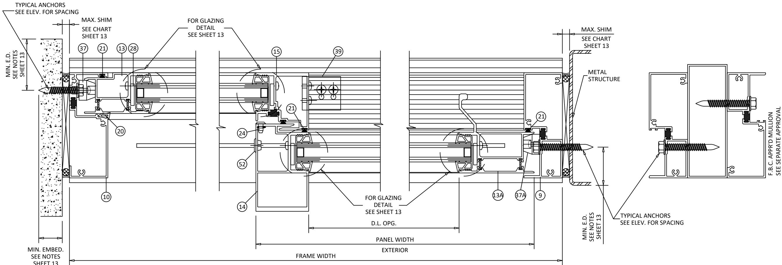
E HORIZONTAL SECTION 9 JAMB - THROUGH FRAME FIXED PANEL - STANDARD SILL
