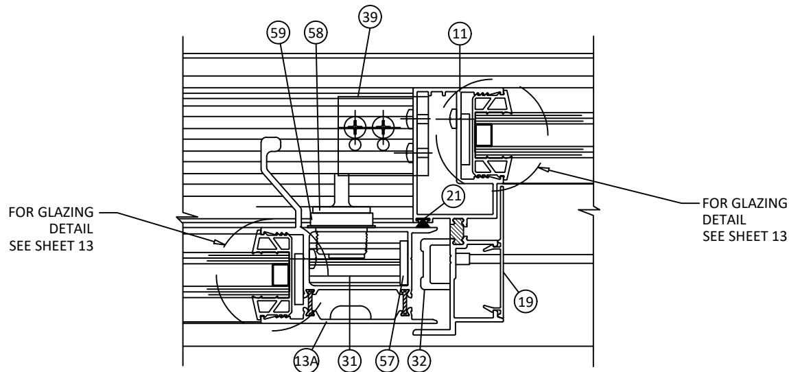
Q HORIZONTAL SECTION INTERLOCK OPERABLE TO FIXED WITH LOCKING HARDWARE STANDARD SILL
