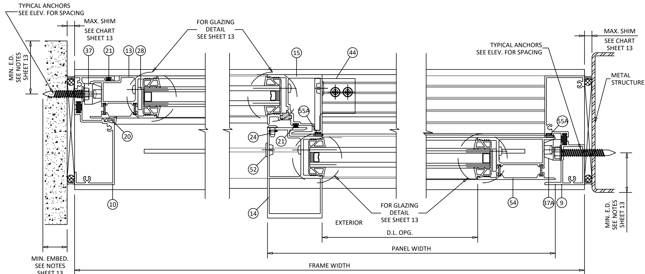
I 10 HORIZONTAL SECTION JAMB - THROUGH FRAME FIXED PANEL - LOW SILL
