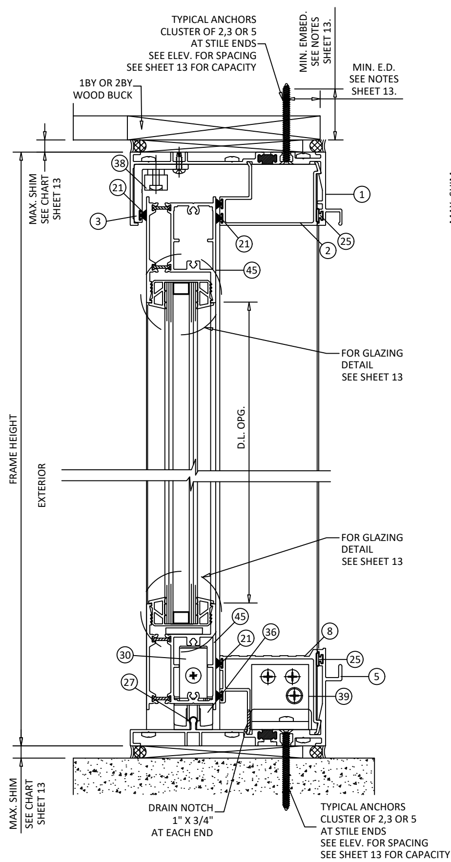
B 7 VERTICAL SECTION OPERABLE PANEL - STANDARD SILL
