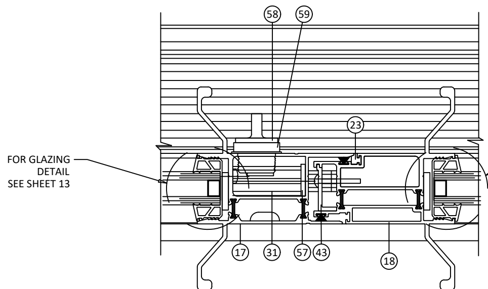
W HORIZONTAL SECTION 12 MEETING STILE WITH LOCKING HARDWARE - STANDARD SILL
