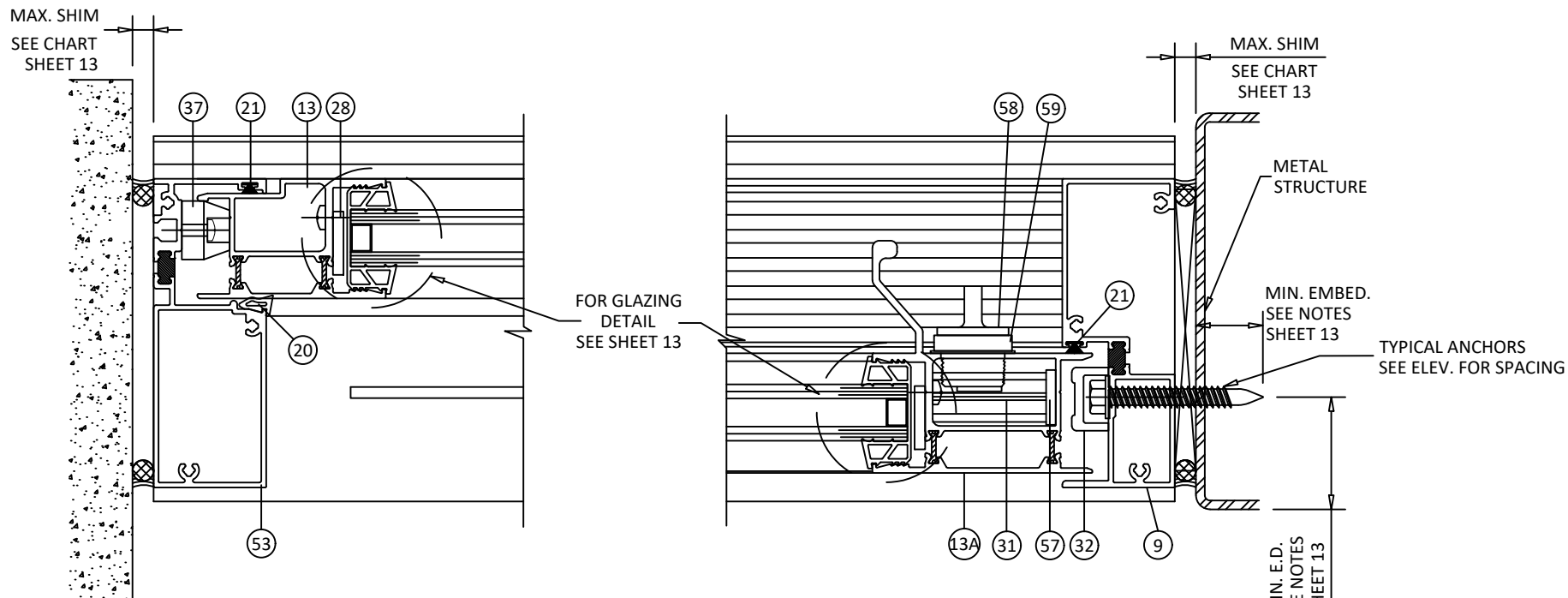
E1 HORIZONTAL SECTION 9 FREE JAMB FIXED PANEL - STANDARD SILL
