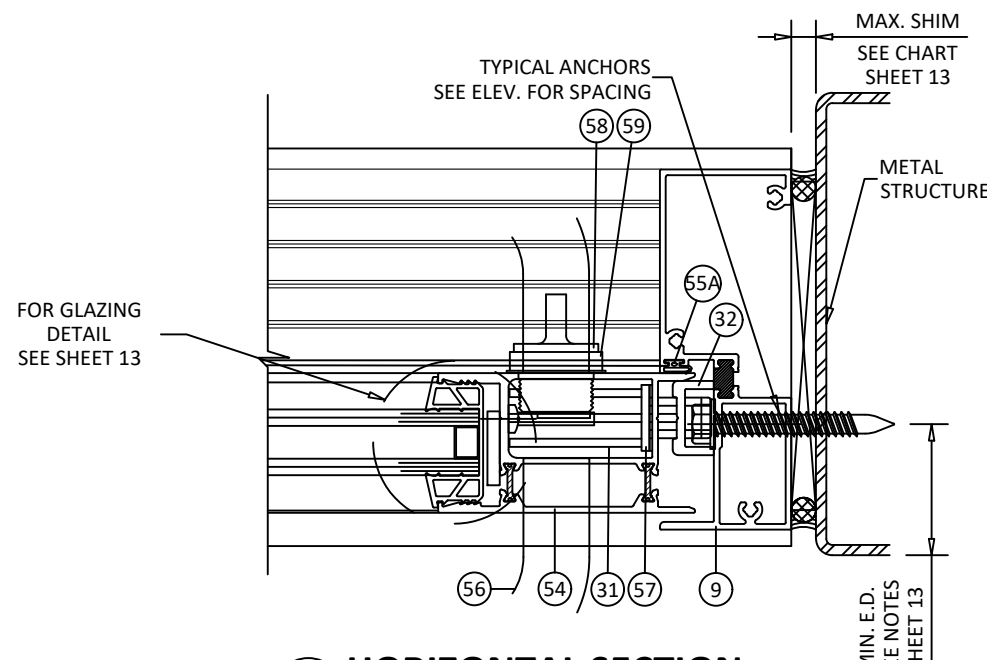
L 10 HORIZONTAL SECTION JAMB - OPERABLE PANEL WITH LOCK HARDWARE LOW SILL
