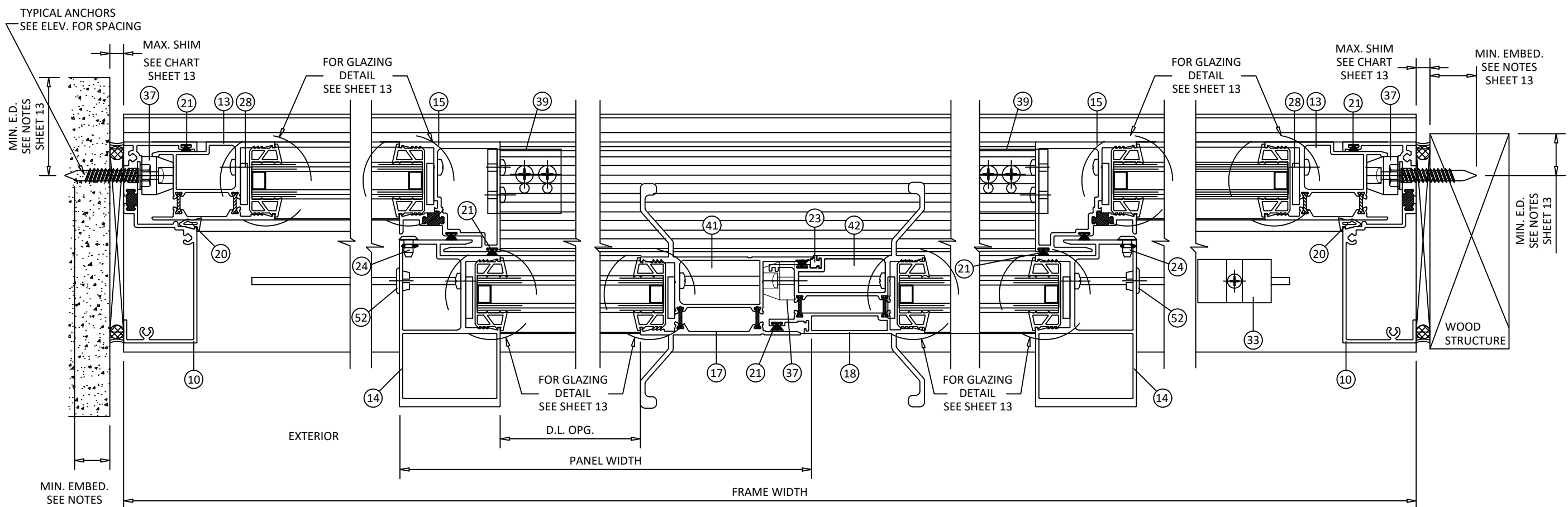
R HORIZONTAL SECTION 12 JAMB - THROUGH FRAME FIXED PANEL - STANDARD SILL S HORIZONTAL SECTION 12 INTERLOCK - FIXED TO OPERABLE STANDARD SILL T HORIZONTAL SECTION 12 MEETING STILE STANDARD SILL U HORIZONTAL SECTION 12 INTERLOCK - OPERABLE TO FIXED STANDARD SILL V HORIZONTAL SECTION 12 JAMB - THROUGH FRAME FIXED PANEL - STANDARD SILL
