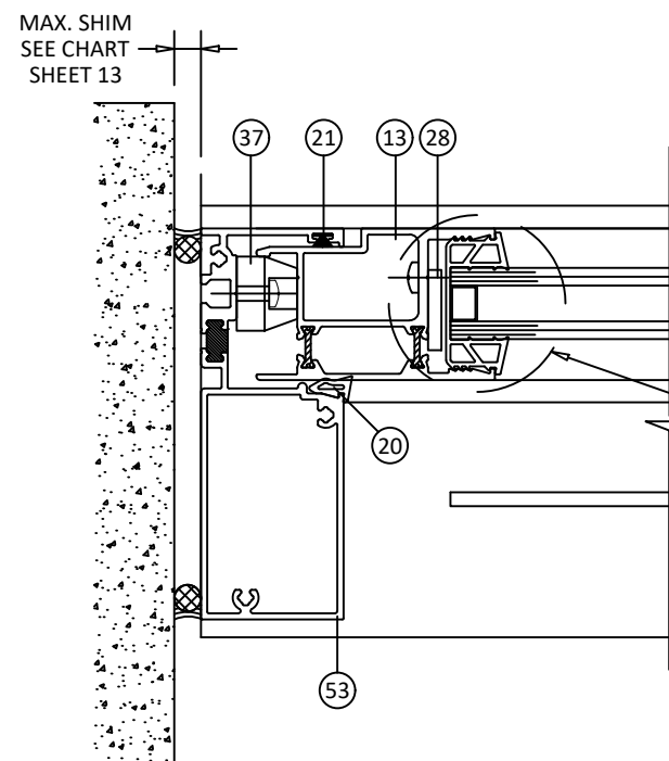
I1 10 HORIZONTAL SECTION FREE JAMB FIXED PANEL - LOW SILL
